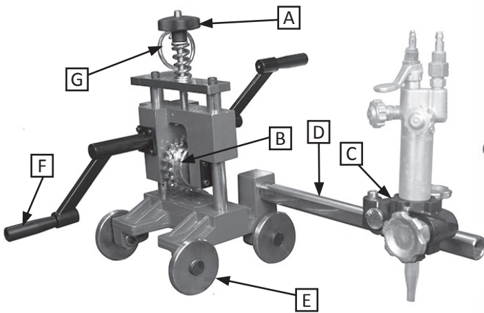
Chain Beveling Machine
